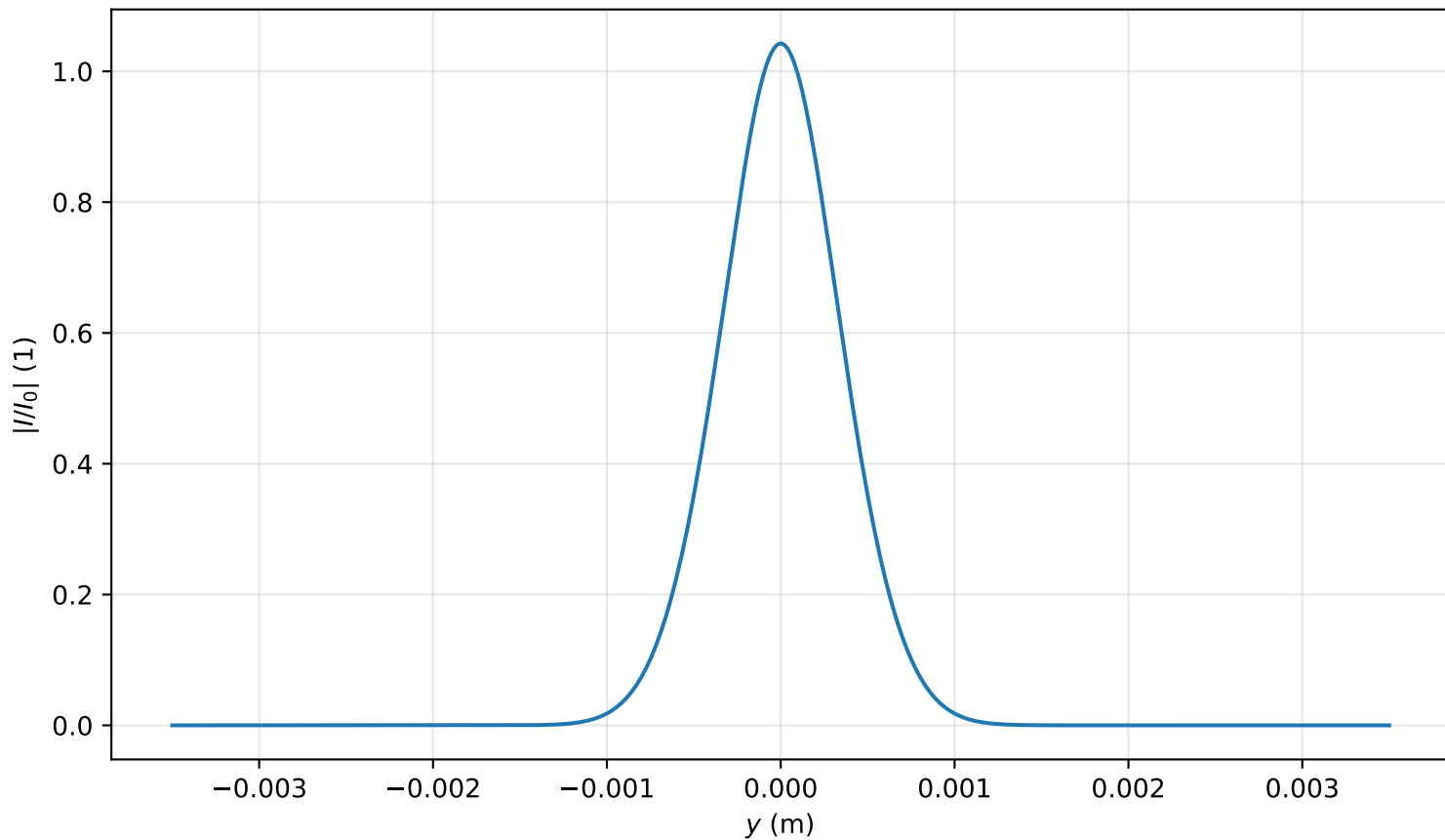
Intensity profile I(x=0, y, z=0.318)/I_0 , P_{in}=0.7P_{cr} , artificial time
